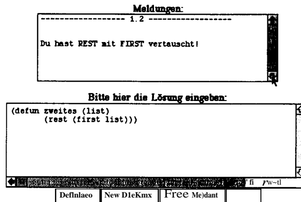
Figure 4: Response of the intelligent diagnosis for an erroneous solution for the problem ZWEITES . The error was caused by the swapping FIRST and REST . This is reported in the upper box "Meldungen."
