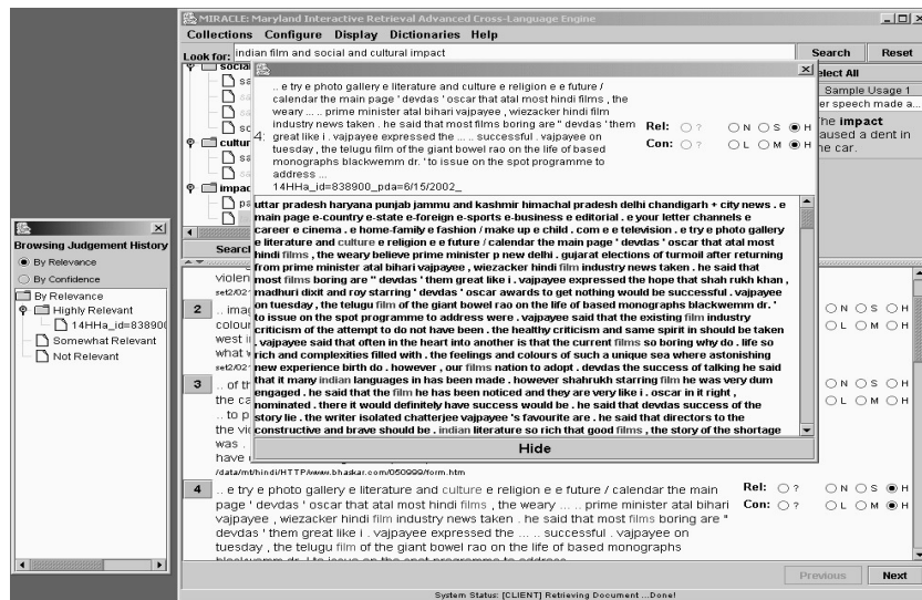
Fig. 6. Document selection and relevance judgments in MIRACLE CLIR system for Hindi. The pop-up window at the center is the full document view window. The pop-up window at the bottom left corner is the judgment history window.
