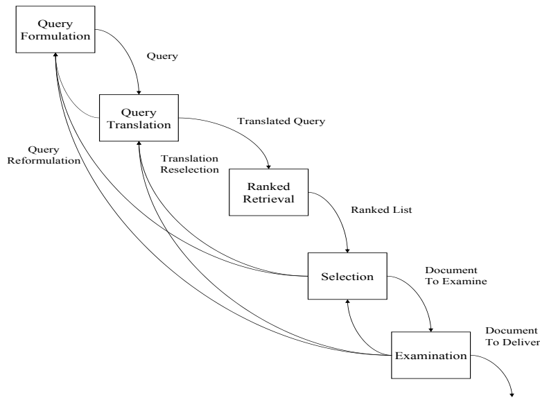
Fig. 1. MIRACLE interaction design. The four interaction points are query formulation, query translation, selection, and examination. Ranked retrieval is a fully automatic process.
