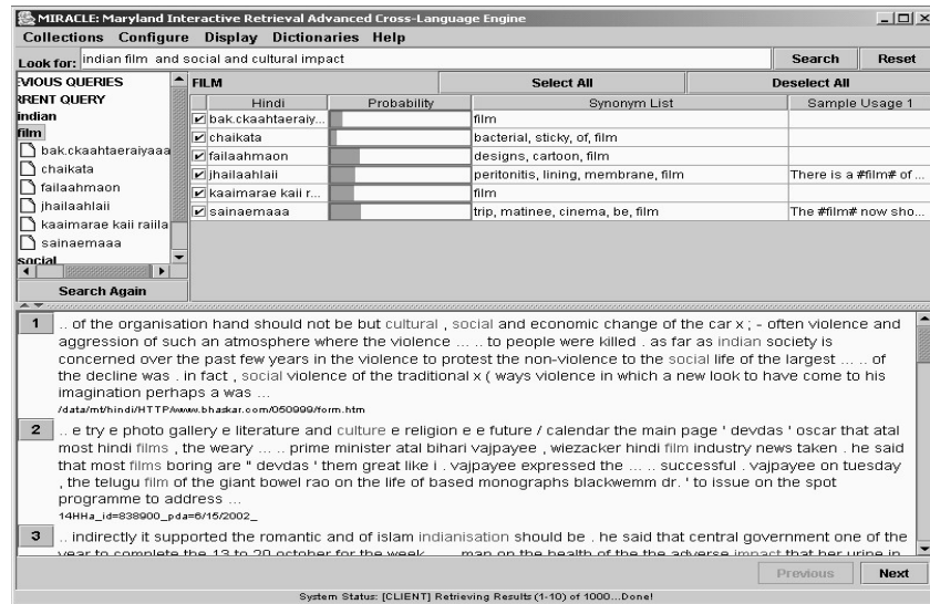
Fig. 4. MIRACLE CLIR system for Hindi
