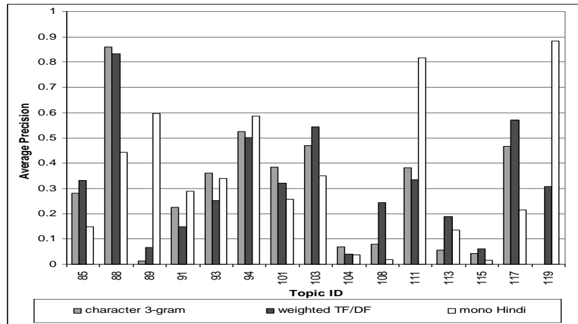
Fig. 7. Summative evaluation results, as reported by NIST, uninterpolated average precision by topic. for one-best 3-grams, word-based weighted structured queries, and monolingual Hindi.
