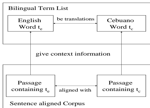
Fig. 3. Constructing cross-language KWIC using a sentence-aligned parallel corpus.
