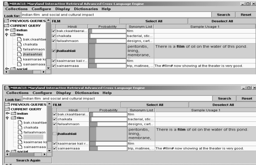
Fig. 5. Translation Selection in the Hindi MIRACLE system. Top: before deselection, bottom: after deselection.
